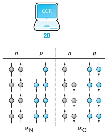
FIGURE 11-3 Mirror nuclides. If all the neutrons are changed to protons and all the protons are changed to neutrons, ^{15}\text{N} becomes its mirror, ^{15}\text{O} . The ground-state energy of mirror pairs differs only in the electrostatic energy.
